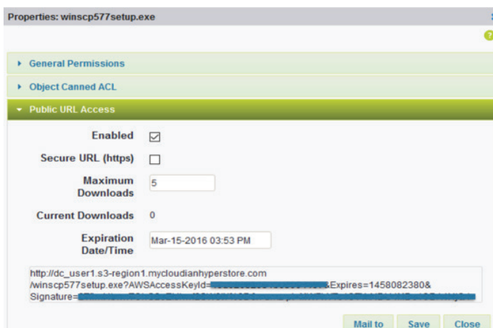
Fig. 1 winscp577setup
